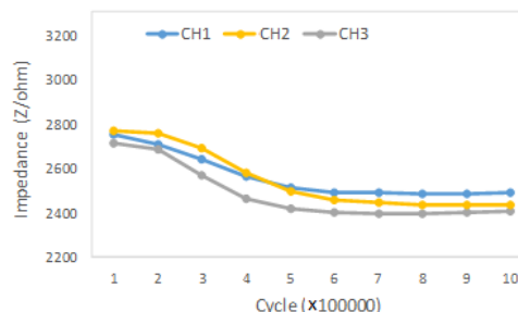
Figure 2: Impedance changes during 1 million cycles of sinusoidal current injection.
