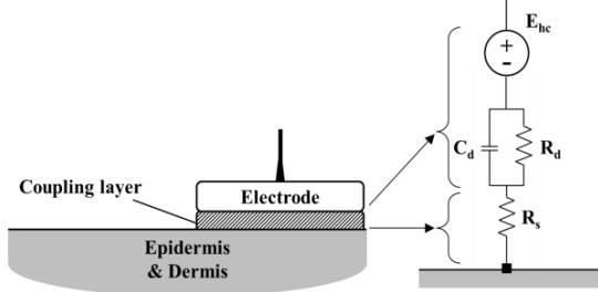
Figure 1: R-C model of skin-electrode interface impedance
