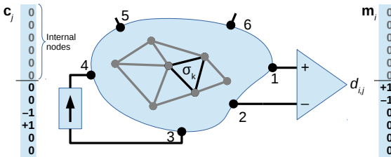
Figure 1: FEM with six electrodes and internal nodes, using current pattern \mathbf{c}_j and measurement pattern \mathbf{m}_i . Electrode nodes are enumerated after internal FEM nodes in this example.
