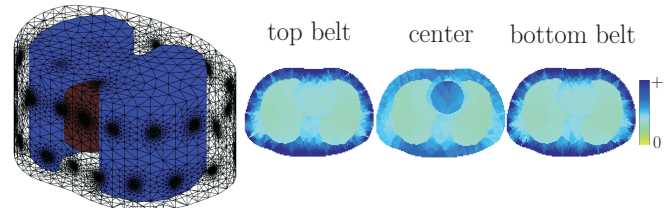
Figure 1: Finite-Element model used in this study (left) and sensitivity distribution in three image planes (right).
