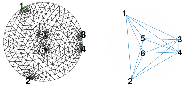
Figure 1: (left) 2D FEM simulation mesh and (right) reduced model as a 15 resistor (blue), 6 terminal (numbered) network, a diode is inserted between terminals #5 and #6 in the interior
