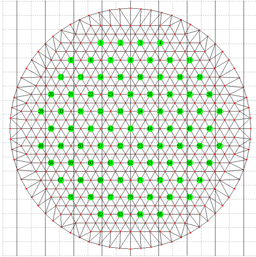
Figure 1: 2D mesh
