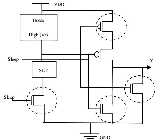
Fig. 2. MTNCL gate structure
