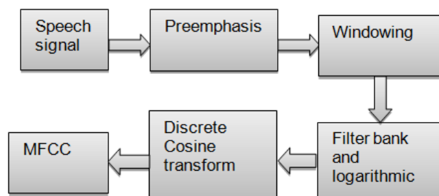
Fig. 1. Feature extraction process of MFCC
