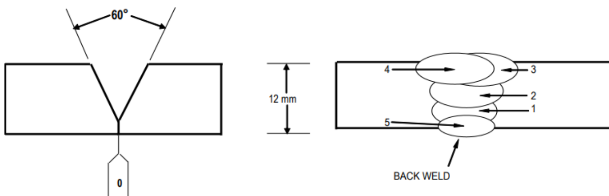
Fig. 1 Weld joint design and weld bead sequence
