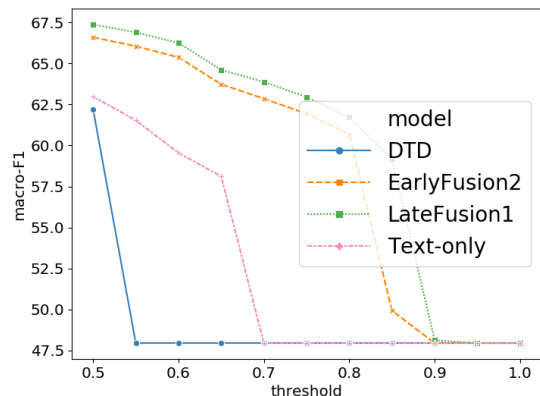
Figure 4: Confidence of the top performing models.
