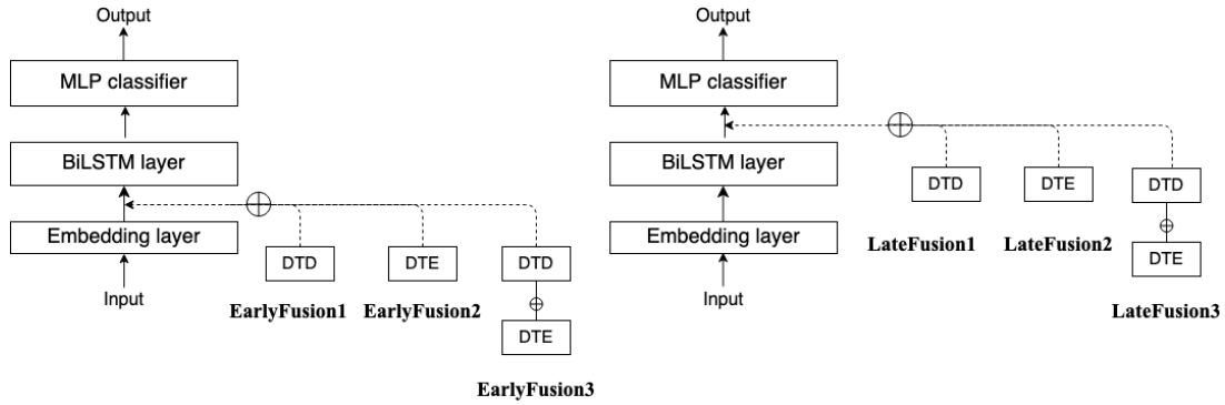
Figure 3: Architectures combining text and topic features.
