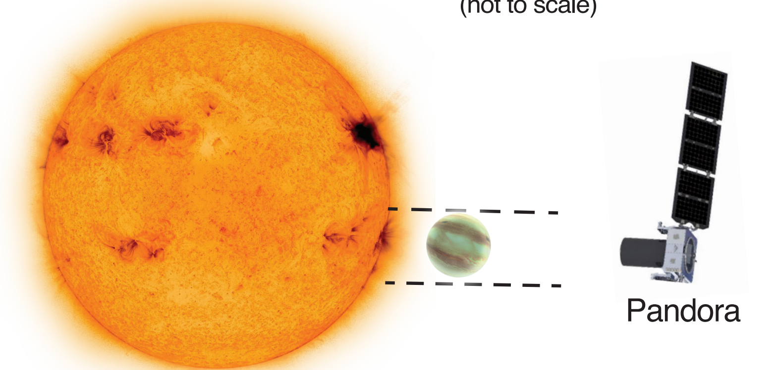
Figure 1: Spectral features from the unocculted stellar regions contribute to stellar contamination of the transmission spectra, which Pandora is designed to measure.
