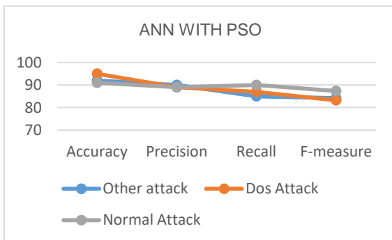
Figure 6: Analysis of ANN_PSO
