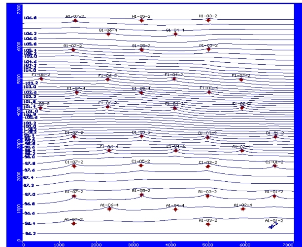
Fig. 8. GPL Map at year 2015, from MODFLOW, for Q_{well} = -1000\ m^3/d
