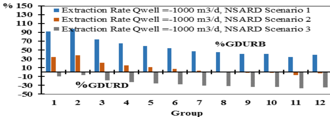
Fig. 11. %GDURB and %GDURD for Q_{well} = -1000 m 3 /d
