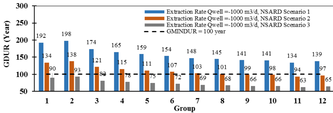
Fig. 10. GDUR under the stress of the minimum considered extraction rate Q_{well} = -1000 m 3 /d
