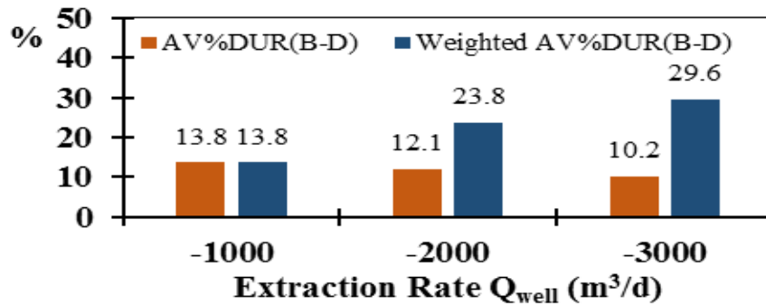
Fig. 16. AV%DUR(B-D) and Weighted AV%DUR(B-D) for the sustainable extraction rates
