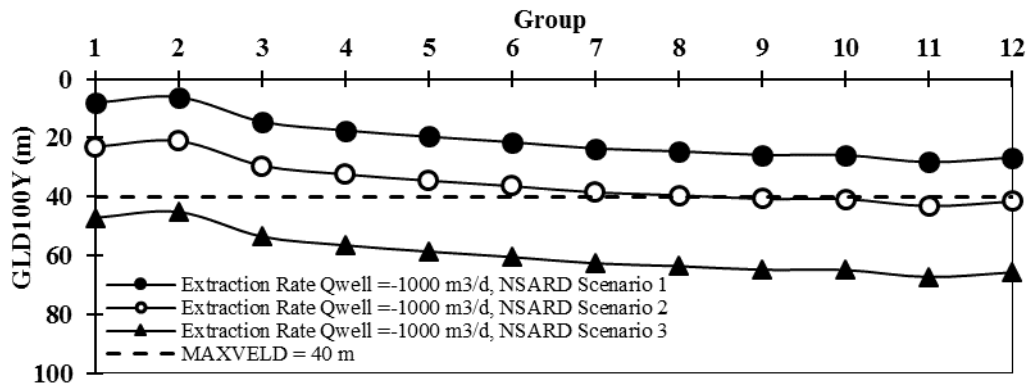
Fig. 13. GLD100Y under the stress of the minimum considered extraction rate Q_{well} = -1000 \text{ m}^3/\text{d}
