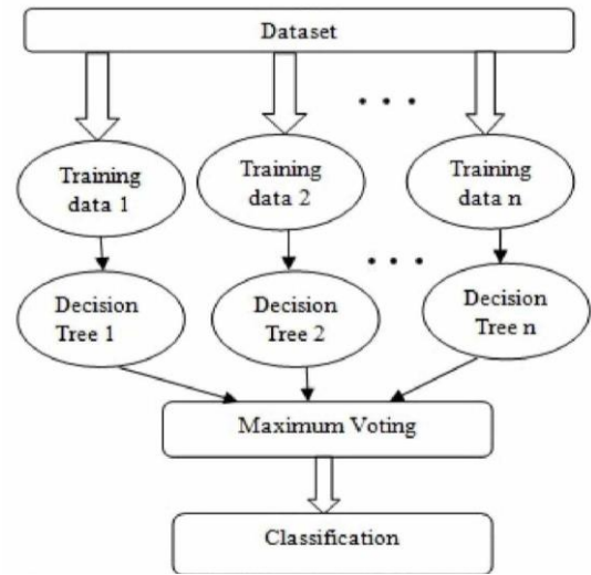
Fig. 4. Random forest
