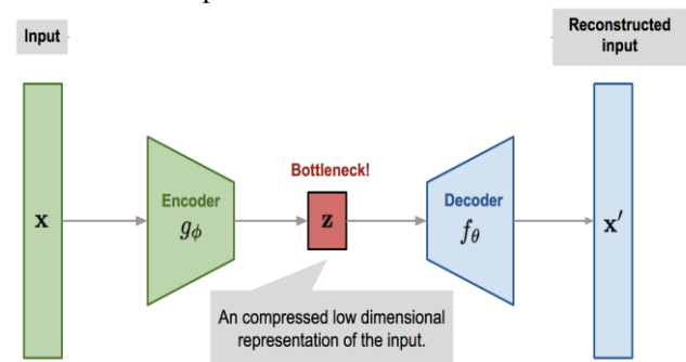
Figure 1: Auto-Encoder [7]
