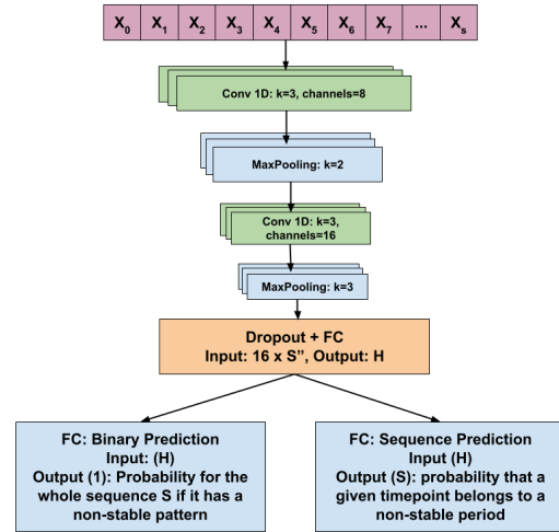
Figure 4: CNN network architecture. Where k is the kernel size, H is the hidden size, and S'' is the length of sequence layers after going through the convolutional layers.
