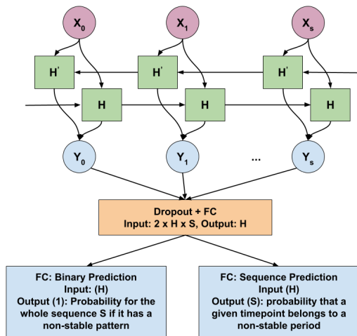
Figure 3: RNN network architecture with biLSTM layer. The prediction Y from all timesteps are used for the FC layer.
