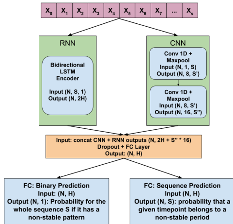
Figure 5: Combined (RCNN) network architecture. Where N is the batch size, H is the hidden size. S is the length of input sequence, S'' is the length of CNN output. The hidden states from LSTM are used for the next layer instead of the predicted outputs.
