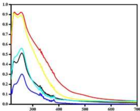
Figure 2: Reflection coefficient of Osmium Dioxide ( \text{OsO}_2 ) and Osmium Tetroxide ( \text{OsO}_4 ) thin films with Os concentrations of (a) 0.5%, (b) 1%, (c) 1.5% and (p) pure sample.
