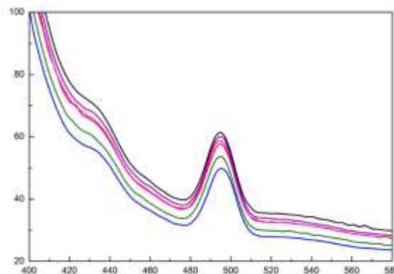
Figure 2: Reflection coefficient of Rhodium (III) Oxide or Rhodium Sesquioxide (Rh 2 O 3 ) and Rhodium (IV) Oxide (RhO 2 ) thin films with Rh concentrations of (a) 0.5%, (b) 1%, (c) 1.5% and (p) pure sample.
