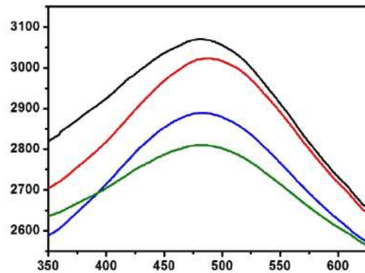
Figure 3: Extinction coefficient of Ruthenium (IV) Oxide (RuO 2 ) and Ruthenium (VIII) Oxide (RuO 4 ) thin films with Ru concentrations of (a) 0.5%, (b) 1%, (c) 1.5% and (p) pure sample.
