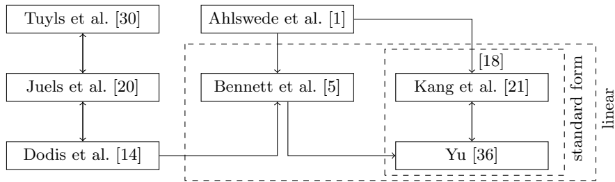
Fig. 11. Pairwise min-entropy loss equivalencies among seven sketches, as indicated by the arrows. Transitive relations apply when following the arrows. E.g., the schemes of Dodis et al. and Kang et al. are equivalent, given that both are instantiated with a linear code in standard form.
