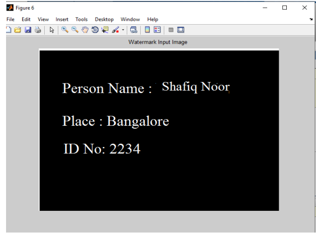
Figure 4: Watermark
