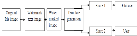
Figure 1: Enrollment module
