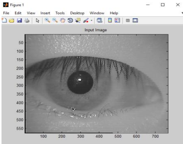
Figure 3: Original Image
