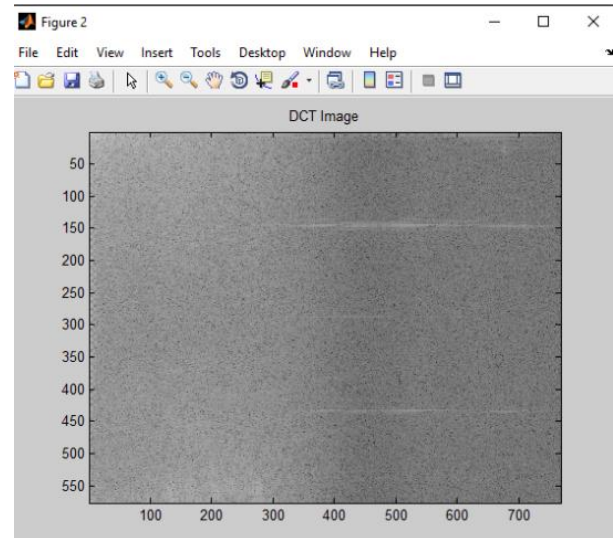
Figure 5: DCT Output
