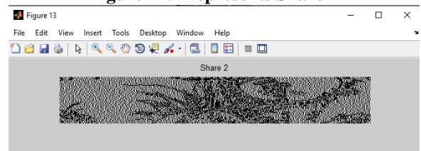
Figure 13: Represents Share 2
