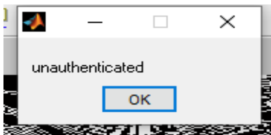
Figure 16: Unauthentication displayed
