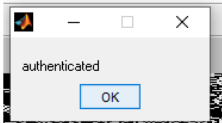
Figure 15: Authentication Displayed
