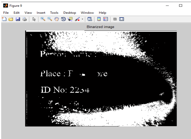
Figure 9: Binarized Image
