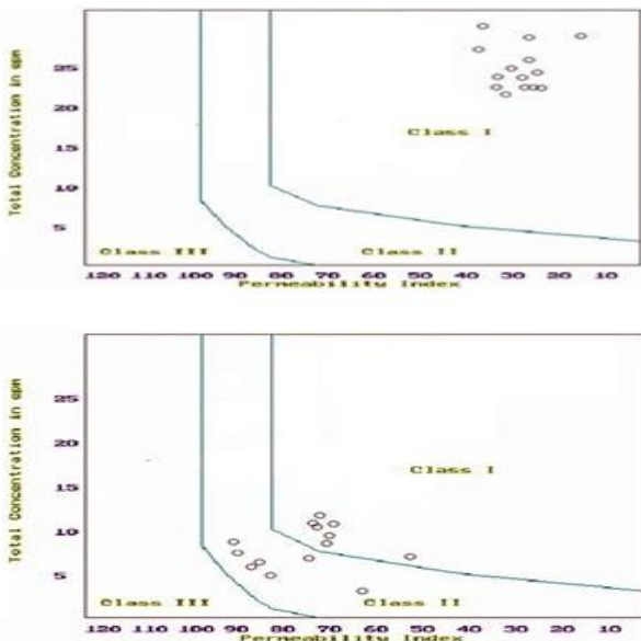
Fig. 8 Classification for irrigation water for soil of medium permeability (Domean, 1964)
