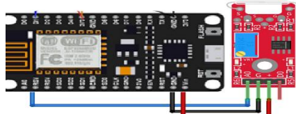
Fig. 8. LM393 Sound Sensor interface
