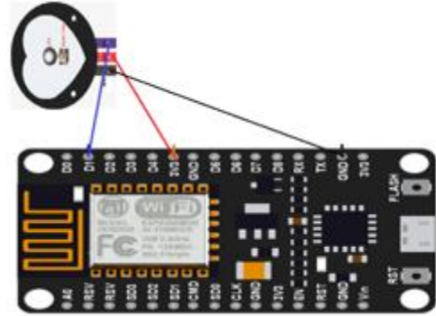
Fig. 5. Pulse sensor interface
