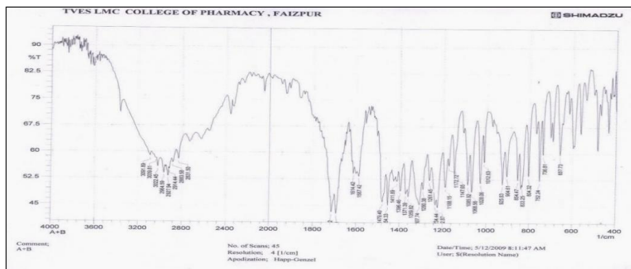
Figure No. 2: FT-IR of spectra physical mixture
