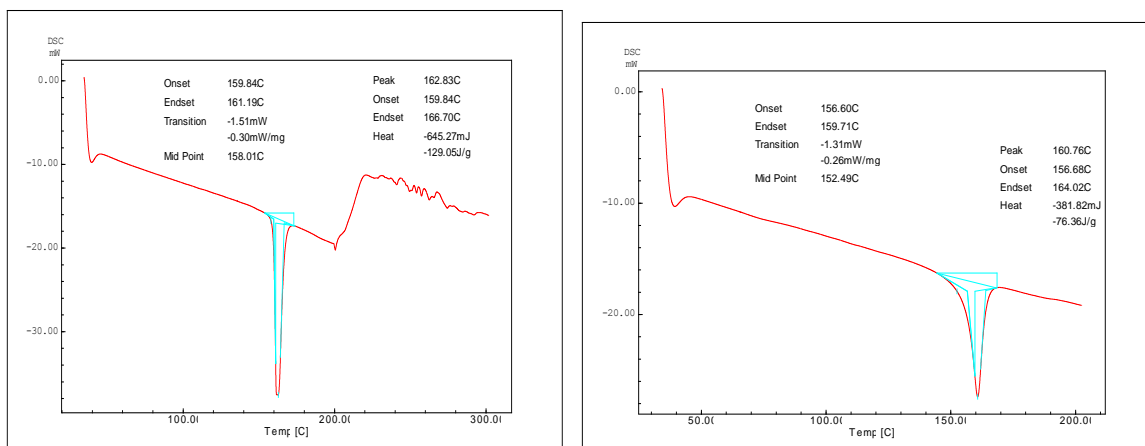
Figure No. 3: DSC thermogram of microspunge formulation
