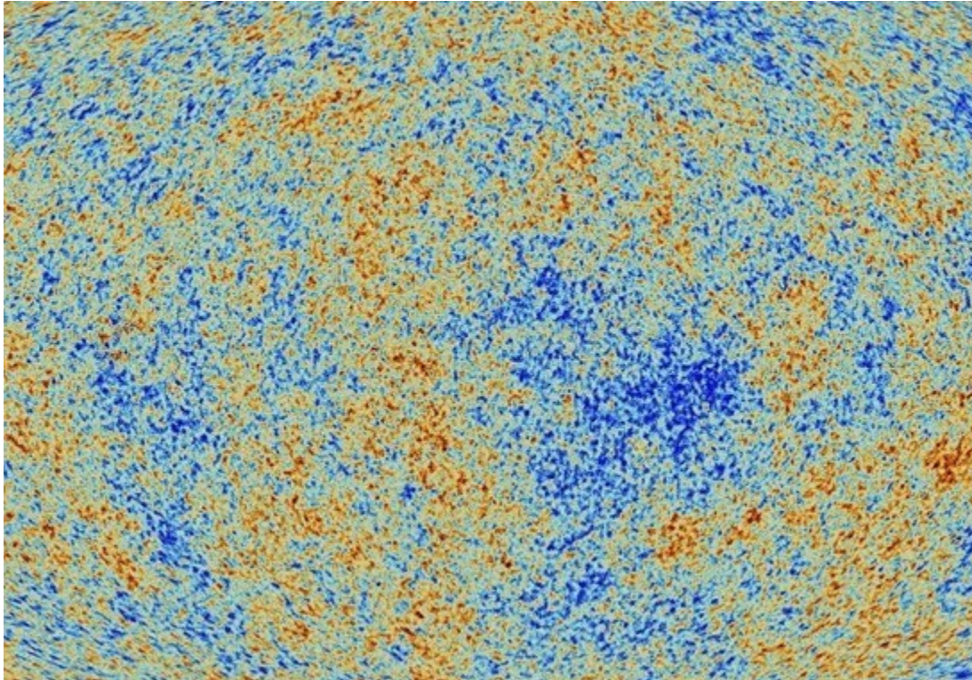
The cosmic microwave background radiation
