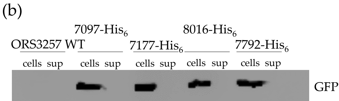
Figure S1. Western blot analysis of effectors in cell-associated and supernatant proteins of ORS3257 WT and \Delta T3SS strains. (a) Western blots were performed with an anti-His 6 antibody. The gene accession number corresponding to the tagged protein for each strain is indicated on the right and the size of the band on the left. (b) Western blot with anti-GFP antibody of cells and supernatant (sup) proteins of ORS3257 WT and strains producing His 6 tagged proteins. The gene number corresponding to the tagged protein for each strain is indicated.
