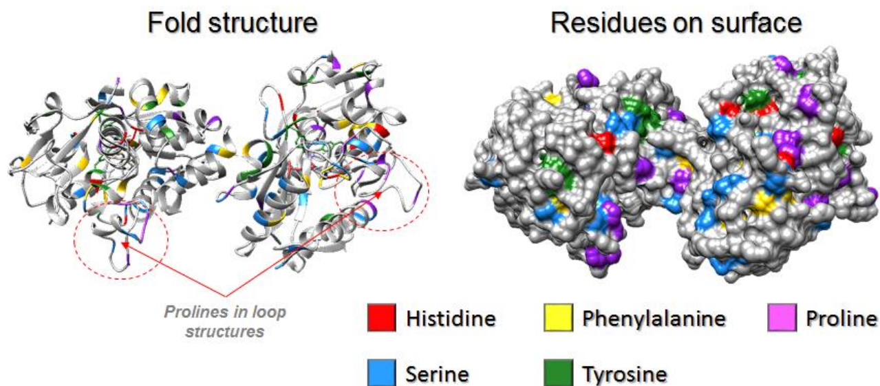
Figure 6. Selected amino acid residues highlighted on the surface of the folded Conalbumin (PDB ID: 2D3I) using Chimera™ software.
