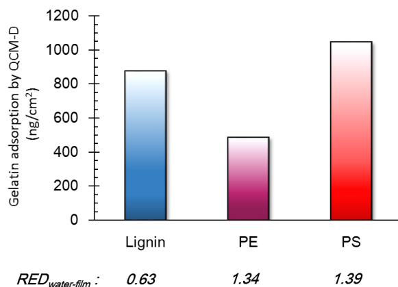
Figure 5. Gelatin adsorption on different films with varying hydrophobicity and surface functionality, as analyzed by QCM-D. Relative energy differences ( RED_{\text{water-film}} ) were calculated using Hansen solubility parameters to indicate the relative hydrophobicity of the three films. For clearly hydrophobic films the RED value is > 1 . (Section SI6 of the Supporting Information for more details).
