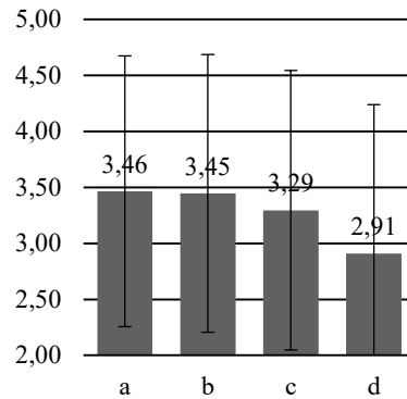
Figure 6: Comparison of the quality of synthesis obtained in different conditions, rescaled to 5.00: (a) Synthesis by the baseline model 1 trained on all available data for M1 or F1 without further adaptation; (b) Synthesis by the proposed model using embeddings corresponding to M1 or F1 without further adaptation; (c) Synthesis by the proposed model after both phases of adaptation to 10 minutes of speech data from M4 or F4; (d) Synthesis by the proposed model after both phases of adaptation to 0.5 minutes of speech data from M4 or F4.
