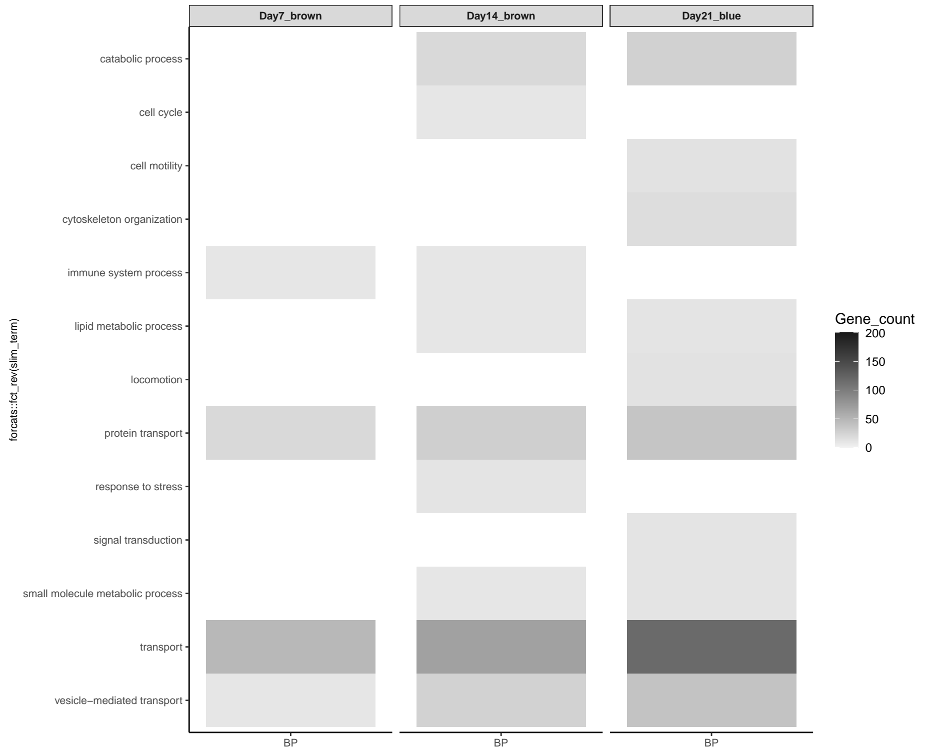
GOslim Biological Process: WGCNA all modules Ambient > Moderate
