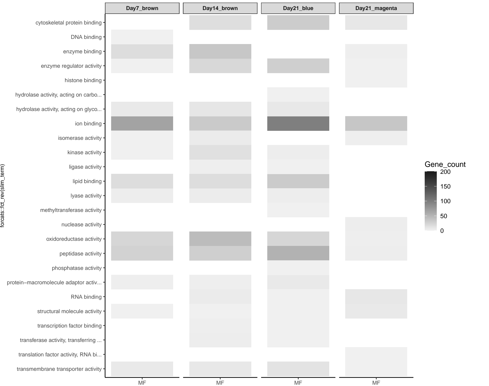
GOslim Molecular Function: WGCNA all modules Ambient > Moderate
