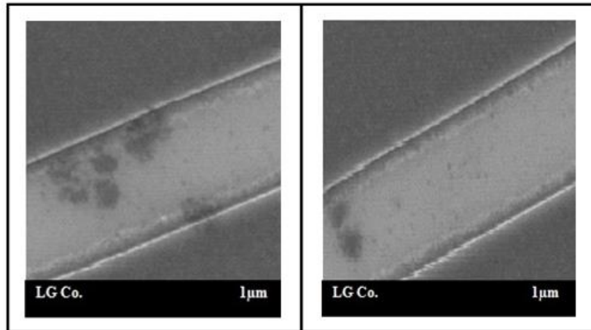
Fig. 6. MEMS microconnections dirty by dust from the interior of the evaluated industry
