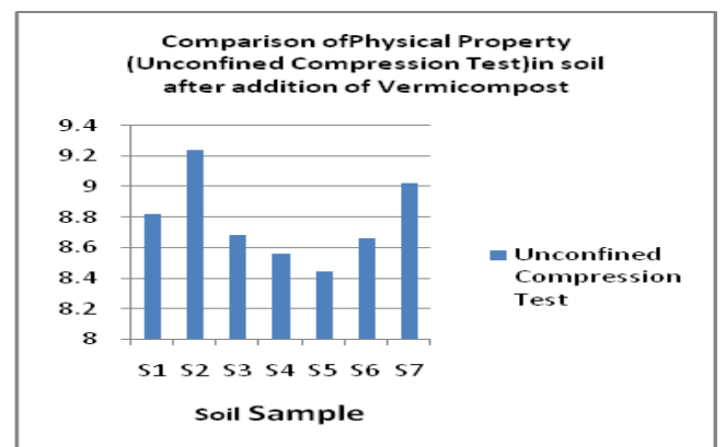
Fig 9 Comparison of Physical property (Unconfined Compression test) in Soil Samples after addition of vermicompost
