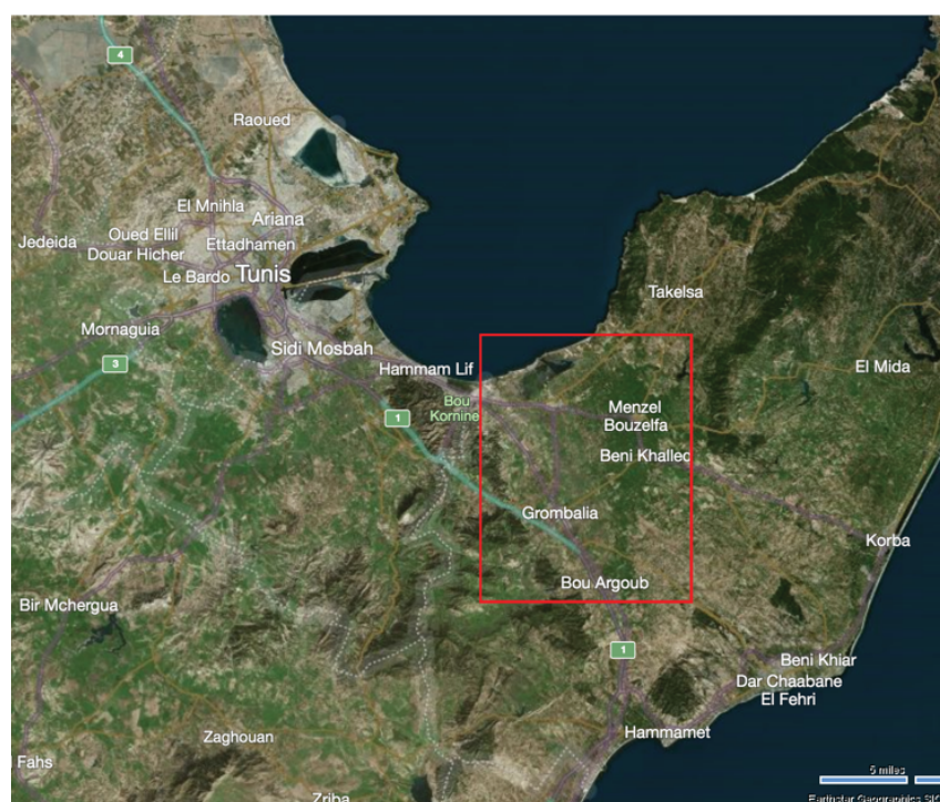
Figure 15. Geographic location of Grombalia Region, Tunisia (Google earth credit)
