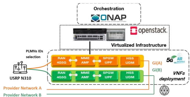
Figure 2. 5G testbed for programmable infrastructure orchestration using ONAP
