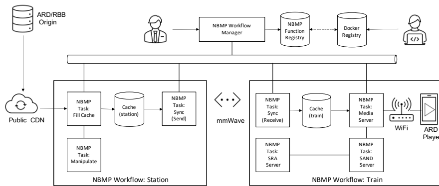
Fig. 3 NBMP Enabled Data Shower Architecture
