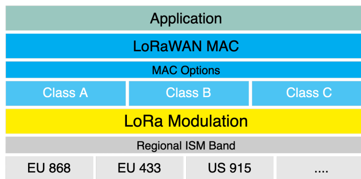
Figure 3. LoRaWAN and LoRa ISO/OSI model layers.
