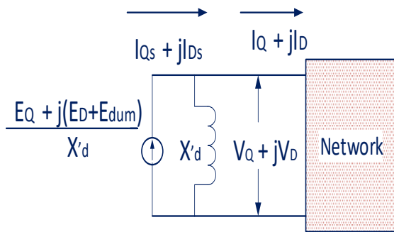
Fig. 2 Generator Representation on Network Side
