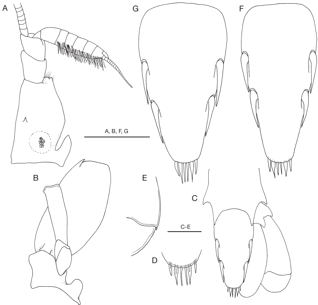
FIG. 2. — Pontonia panamica n. sp.: A , antennule, ventral view; B , antenna, ventral view; C , telson and uropods, dorsal view; D , posterior margin of telson, dorsal view; E , distolateral margin of uropodal exopod, dorsal view; F , G , telson, dorsal view; A-E , ♀ paratype, pcl 6.0 mm (MNHN-Na 16394); F , ♂ paratype, pcl 4.8 mm (MNHN-Na 16394); G , ♀ paratype, pcl 6.0 mm (USNM 1103080). Scale bars: 1 mm.
