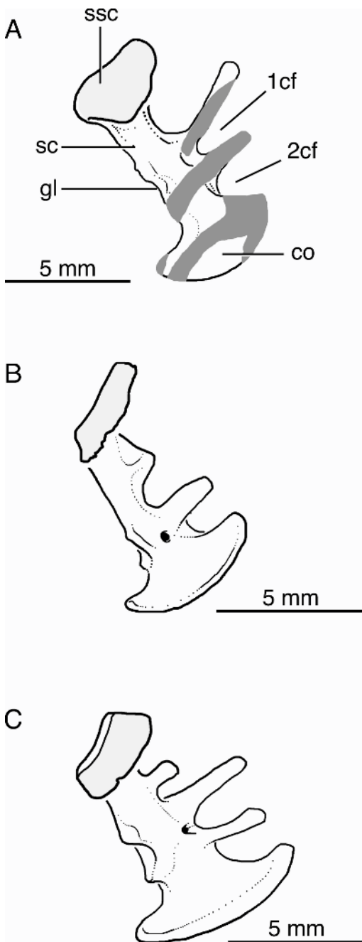
Fig. 13. A, left scapulocoracoid and suprascapula of Saichangurvel davidsoni (IGM 3/858) in dorsal view. Ribs overlie parts of the scapulocoracoid, but these hidden parts are reconstructed in gray; enough of the girdle is visible to confirm the presence of two bars forming the primary (1cf) and secondary (2cf) coracoid emarginations. The suprascapula is shown as
