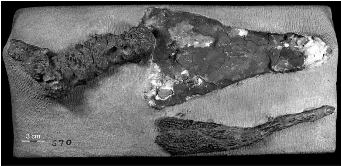
FIG. 1. Panel mount of Eutretauranosuchus delfsi AMNH FARB 570. The skull has been removed, and the right mandible and cervical region remain.
