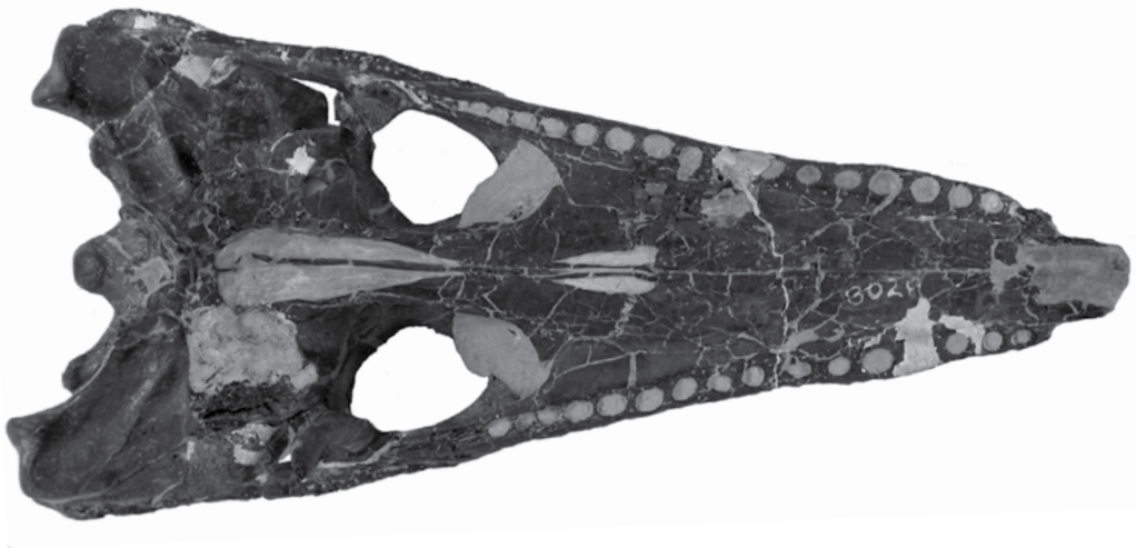
FIG. 3. Holotype of Eutretraurosuchus delfsi CMNH 8028 in (A) dorsal and (B) ventral view.
