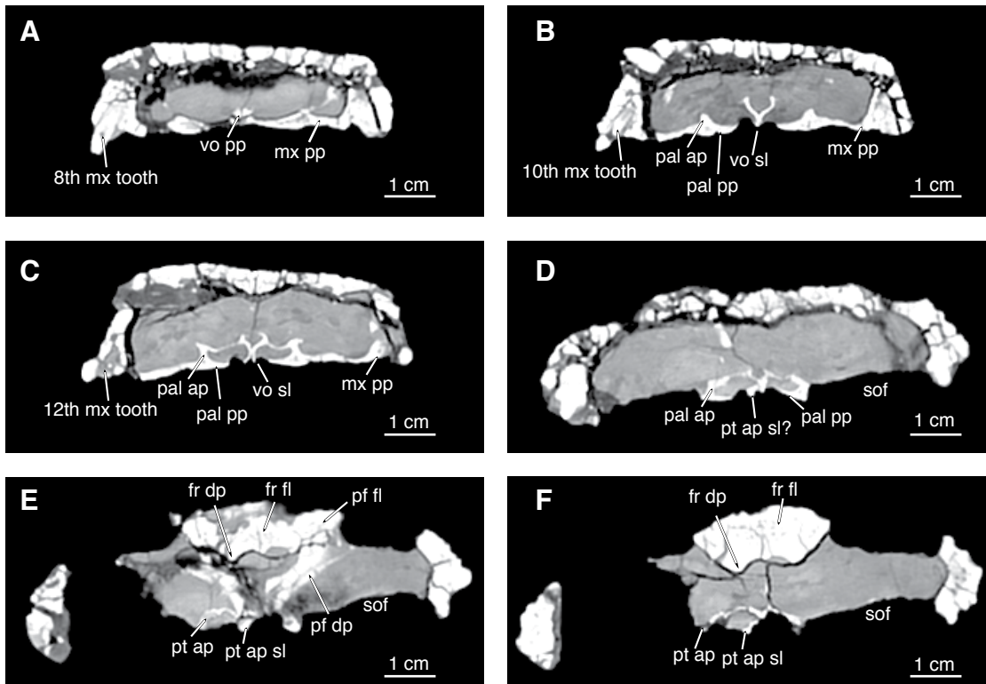
FIG. 8. Transverse CT sections through the skull of Eutretauranosuchus delfsi AMNH FARB 570. (A) Tra 359, (B) Tra 400, (C) Tra 435, (D) Tra 555, (E) Tra 585, (F) Tra 616. See appendix 2 for abbreviations.
