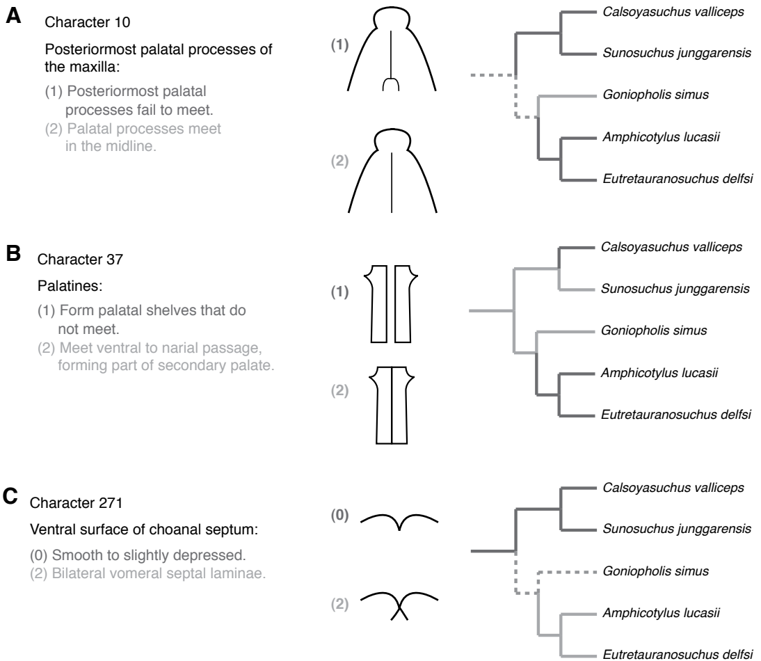
FIG. 20. Tracing of ancestral palatal character states ( A ) 10, ( B ) 37, and ( C ) 271 for Goniopholididae. Each row features a description of the character, a cartoon of relevant character states, and a color-coded phylogeny displaying the distribution of the character within Goniopholididae. The palates illustrated in A and B are drawn in ventral view, whereas the vomeral complex in C is drawn in transverse section. Color-coding on the phylogeny is equivalent to the colors used to indicate relevant states on the cartoons. Dotted lines indicate ambiguous reconstruction.
