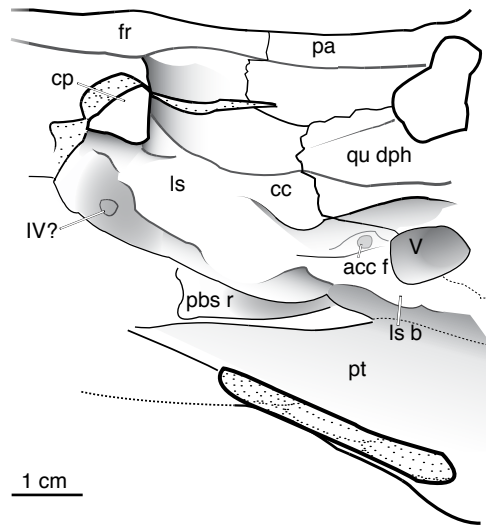
FIG. 11. Braincase of Eutretrauranosuchus delfsi AMNH FARB 570 in left lateral view. See appendix 2 for abbreviations.
