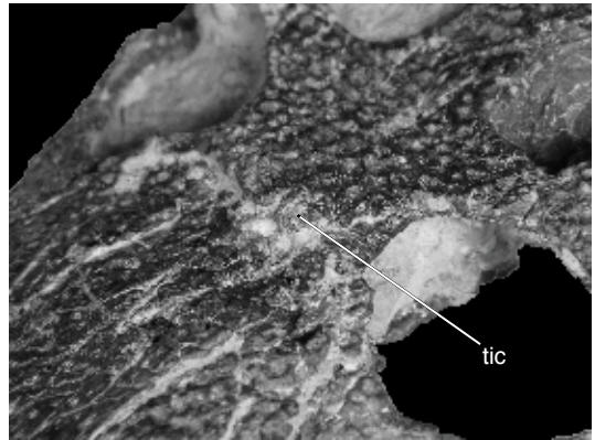
FIG. 9. Eutretauranosuchus delfsi AMNH FARB 570. Interorbital region in oblique dorsolateral view. See appendix 2 for abbreviations.
