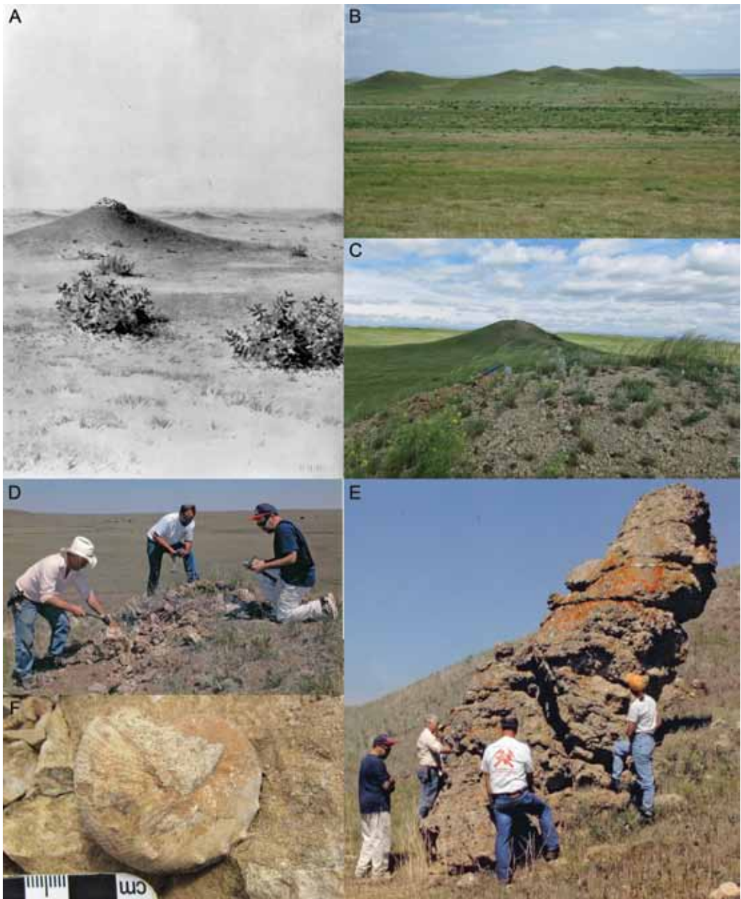
FIG. 2. Tepee buttes in the Pierre Shale of Colorado, Wyoming, and South Dakota. A. Tepee butte along the Front Range of Colorado, as illustrated by Gilbert (1896: pl. 67). B. Overview of tepee buttes at AMNH loc. 3494, Weston County, Wyoming. Photo by S. Klofak. C. Close-up of tepee butte at AMNH loc. 3494, Weston County, Wyoming. Photo by M. Garb. D. Close-up of tepee butte at AMNH loc. 3344, Butte County, South Dakota, with three of the authors for scale. Photo by B. Brown. E. Tepee butte near AMNH loc. 3344, Butte County, South Dakota. The shale surrounding the limestone core of the tepee butte has weathered away, exposing the core. Photo by B. Brown. F. Macroconch of Hoploscaphites gilberti , n. sp., AMNH loc. 3494, Weston County, Wyoming. Photo by M. Garb.
