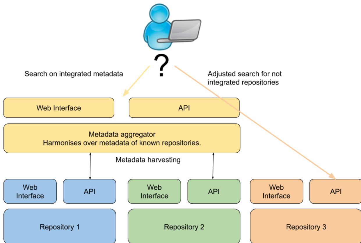
Figure 3: When repositories' metadata is only captured by integrated platforms and not by others, the problem of non-interoperable repositories is only shifted to another layer of the data infrastructure.
