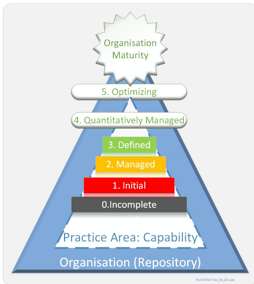
Diagram 7: Tiered Capability/Maturity
