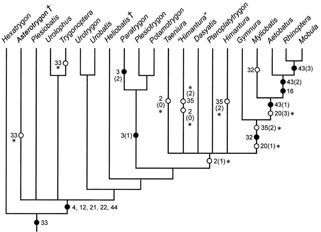
Fig. 44. Tree topology taken from figure 43 (strict consensus tree) with ambiguous characters mapped (numbered as in text and matrix in table 5, unambiguous characters in fig. 43). Some of the characters are ambiguous because they are scored as uncertain in Hexatrygon (characters 4 and 21) and in Myliobatis (character 16); these are displayed conservatively on the tree (i.e., it is not simply assumed that they will be found in these taxa). Other characters have more than one equally parsimonious optimization (characters 3, 20, 32, 43), whereas others are scored as uncertain in the Green River stingrays (characters 12, 22, and 44). The optimization chosen in both of these cases is accelerated transformation, favoring reversals over independent gains. Characters denoted with an asterisk (*) are part of multistate transformation series that have unambiguous character states in figure 43.
