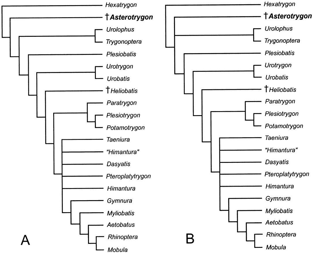
Fig. 45. Five subgroups of trees showing the different phylogenetic positions of † Asterotrygon that result once uncertainty concerning the relationships among dasyatid genera is eliminated from the minimum-length trees obtained in this study (based on matrix in table 5; strict consensus in fig. 43). † Asterotrygon pairs with urolophids in the subgroups depicted in C–E, representing 21 of the 35 equally most parsimonious trees (see text for details).
