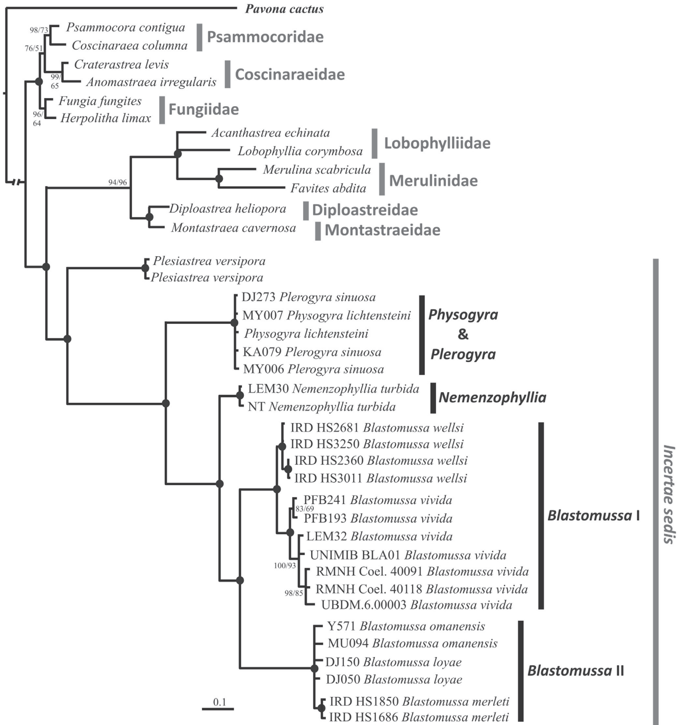
Fig. 5. Phylogenetic tree of rDNA (spanning the entire ITS1, 5.8S, ITS2 and a portion of 28S and 18S) reconstructed with Bayesian Inference. Numbers at each node show percentages of Bayesian posterior probability (>70%) and MP bootstrap (>50%); – = no support. Filled circles indicate well-supported clades (bootstrap values \geq 99 and posterior probability of 100).
