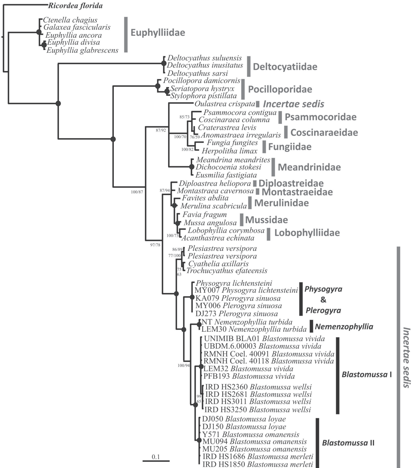
Fig. 4. Phylogenetic tree of mitochondrial gene COI reconstructed with Bayesian Inference. Numbers at each node show percentages of Bayesian posterior probability (>70%) and MP bootstrap (>50%); – = no support. Filled circles indicate well-supported clades (bootstrap values \geq 99 and posterior probability of 100).
