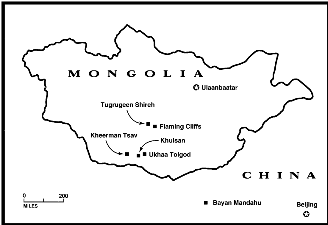
Fig. 1. Map of Mongolian Gobi Desert showing major fossil localities.
