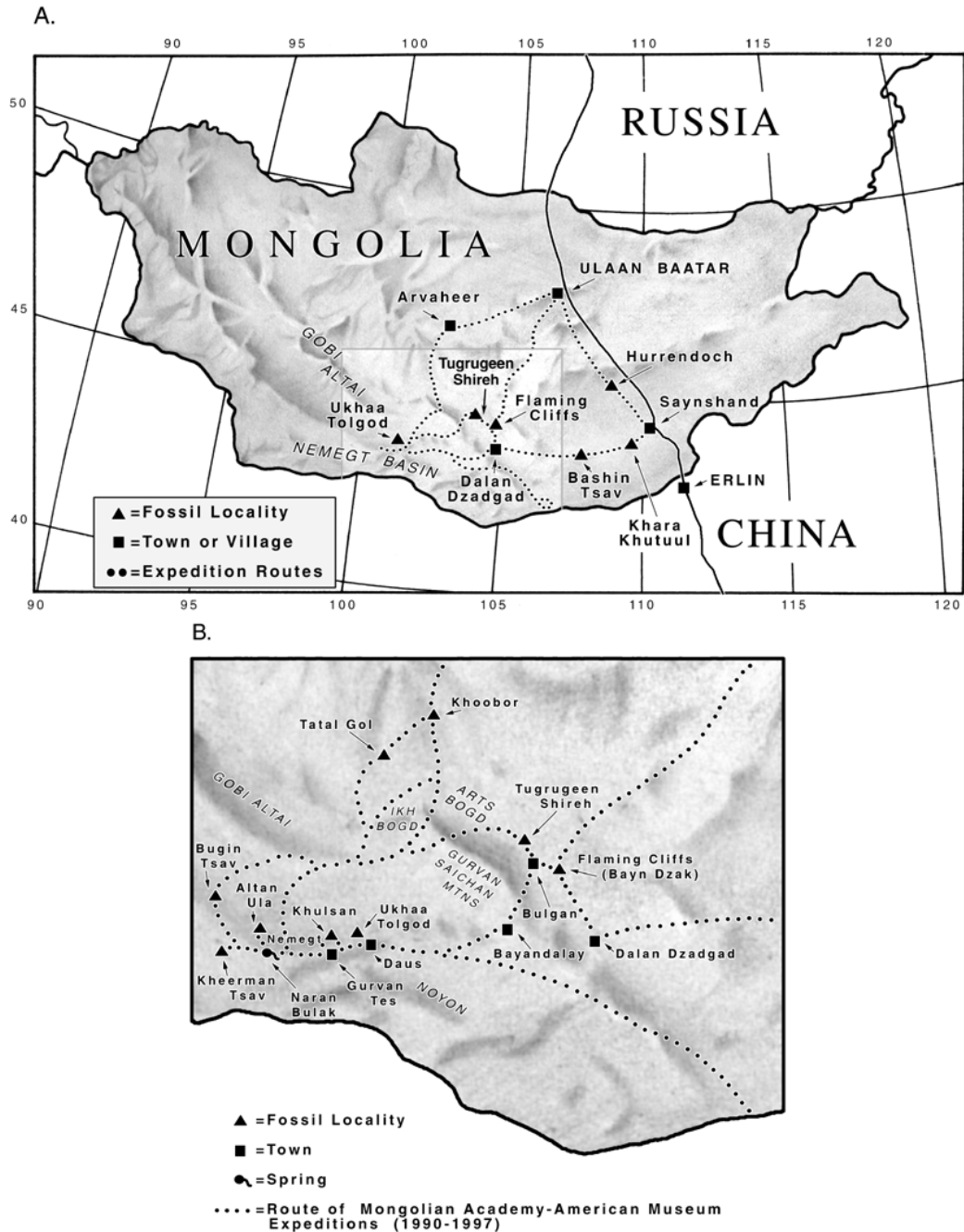
Fig. 1. Map of Mongolia (A) with inset of south-central region (B) indicating the major fossil localities visited by the joint expeditions of the Mongolian Academy of Sciences and the American Museum of Natural History. The specimens of Kryptobaatar dashzevegi described here come from Ukhaa Tolgod and Tugrueen Shireh.
