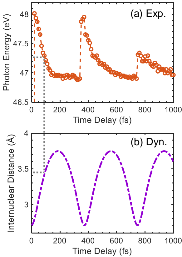
FIG. 7. (a) Photon energy position at the maximum \Delta OD of the feature reflecting the vibrational dynamics in the B^3\Pi_{0^+u} state observed in Fig. 2. (b) One-dimension classical dynamics simulation in the B^3\Pi_{0^+u} excited state.
