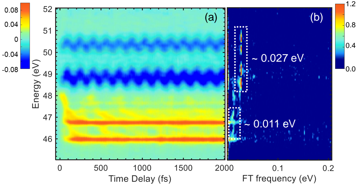
FIG. 3: Measured differential absorption map and Fourier analysis. (a) Measured transient absorption spectra (in \Delta OD ) as a function of the time delay and of the XUV photon energy. (b) Fourier transformation along the time delay abscissa axis of the transient absorption map on panel (a). White dotted boxes highlight the major frequencies observed.
