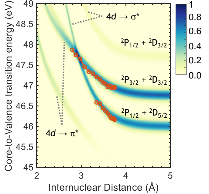
FIG. 8. Computed XUV absorption strengths from the B^3\Pi_{0^+u} state into the core-excited states as a function of the transition energy and the internuclear distance. The color scale shows the normalized transition probability. Orange circles and orange lines: Experimental curve of core level transition energy versus internuclear separation extracted from the experimental transient absorption map.
