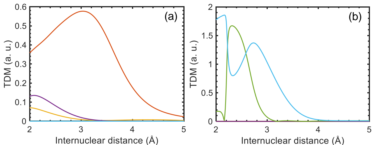
FIG. A1: Computed transition dipole moments (TDM) (a) as a function of the internuclear distance R for one-photon excitation from the I_2 ground state into A^3\Pi_{1u} (yellow line), B''^1\Pi_{1u} (purple) and B^3\Pi_{0+u} (red line) excited states, and (b) TDM for one-photon excitation from the populated B^3\Pi_{0+u} state into the Y^3\Sigma_{0+g}^- (green line) and Z^3\Pi_{0+g} (cyan) excited states.
