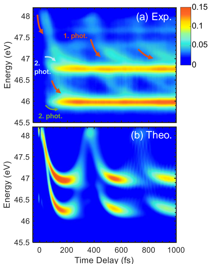
FIG. 5. (a) Experimental transient absorption map (in \Delta\text{OD} ) following \text{I}_2 excitation by the visible pump pulse, as a function of the time delay and the XUV photon energy. Red arrows (labelled 1. phot.) highlight the observed vibrational wave packet motion by one-photon absorption as features significantly moving in energy with time. Green and gray arrows (labelled 2. phot.) indicate additional direct dissociation features due to two-photon excitation in the experimental data (see Fig. 6). (b) Simulated transient absorption (1. phot.) from the wave packet in \text{B } ^3\Pi_{0+u} excited state following one-photon absorption at 520 nm.
