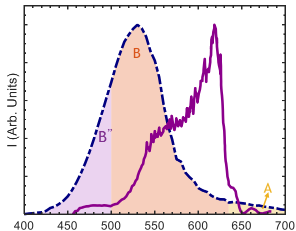
FIG. 2 Absorption spectrum of I_2 , in the visible (blue line) compared to the spectrum characterizing the visible pump pulse (purple line). The spectral region where each excited state, A^3\Pi_{1u} , B^3\Pi_{0+u} and B''^1\Pi_{1u} , absorbs are highlighted by a yellow, orange and violet area, respectively.
