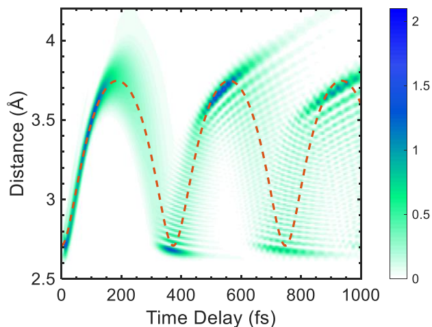
FIG. C3: Nuclear wave packet evolution (colormap) in the B state, following excitation at 520 nm (obtained by numerically solving the TDSE for the nuclear motion) compared with the one-dimension classical dynamics (orange line).
