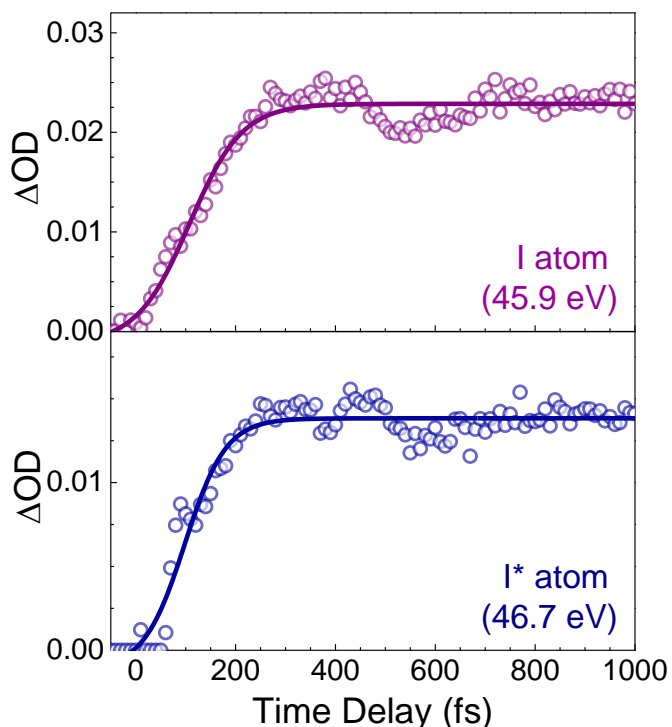
FIG. B1: Measured transient for the dissociation into I and I* atomic fragments. Time traces extracted from Fig. 5 (a): Amplitude of the Gaussians functions (circles) used to describe the features associated with the formation of I and I* at around 45.9 eV and 46.7 eV, as a function of time, and the corresponding fit to a Boltzmann sigmoidal function (line). Both transients are consistent with a fast dissociation with \tau_{\text{diss}} \sim 100 fs.
