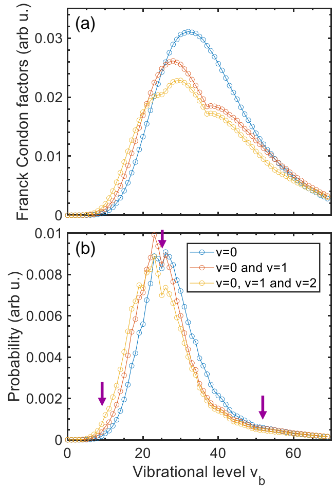
FIG. C1: (a) Computed Franck-Condon factors between the ground state and the B^3\Pi_{0_u}^+ state as a function of the populated vibrational level on the B state. Three initial vibrational populations in the X state are considered: only v = 0 , v = 0 (80%) and v = 1 (20%), and v = 0 (70%), v = 1 (20%) and v = 2 (10%). (b) Corresponding excitation probability using the pump pulse spectrum. Vertical purple arrows indicate the three starting points selected for the classical dynamics (Fig. C2 (b)).
