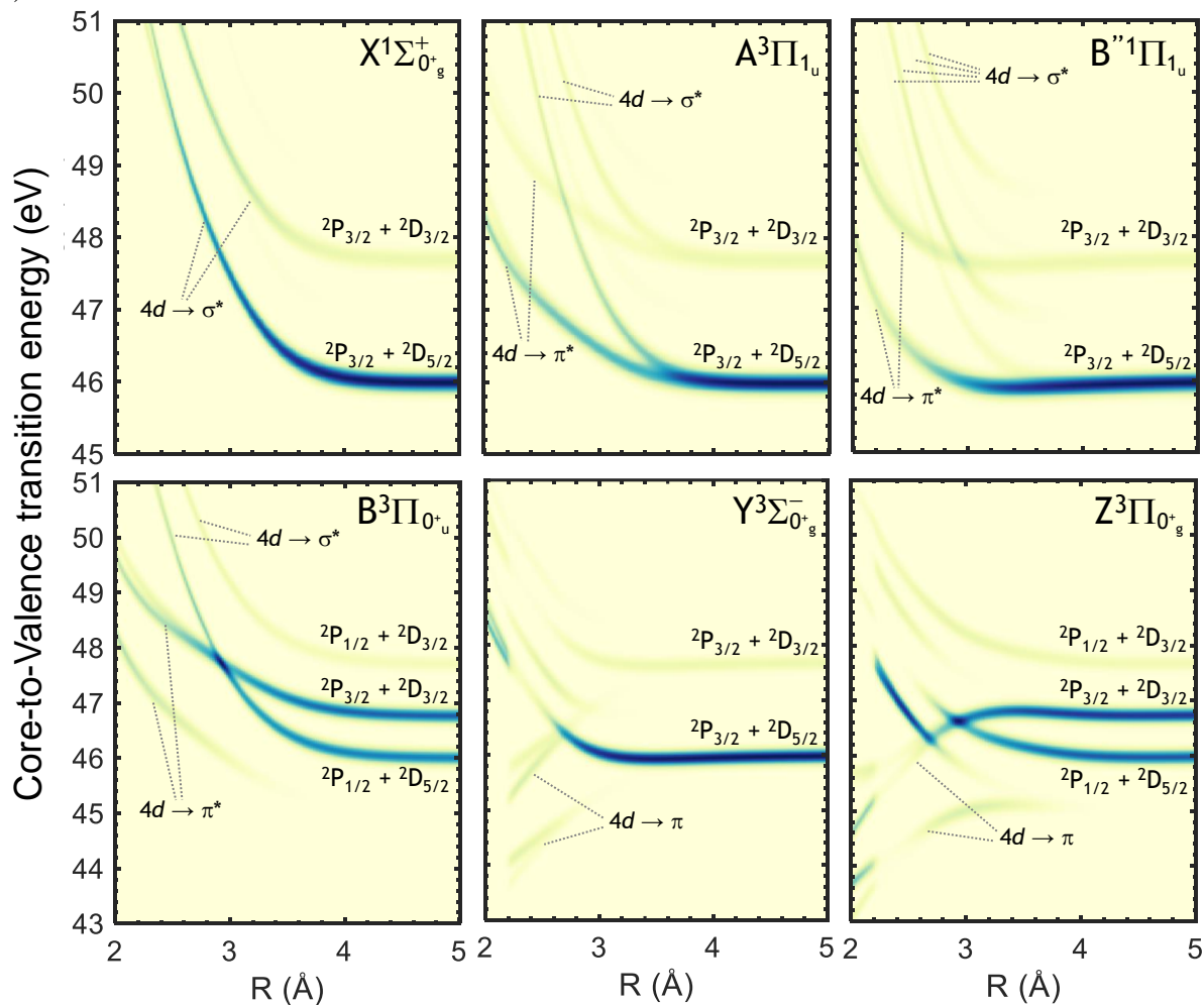
FIG. A2: Computed absorption probabilities between each valence electronic state and the core-hole excited states as a function of the core-to-valence transition energy and the internuclear distance R .
