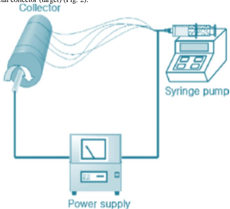
Fig. 2. Diagram of the electro spinning apparatus [19].
