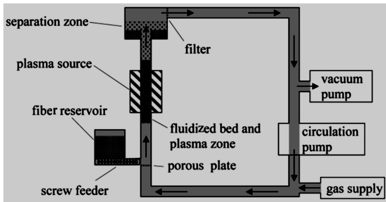
Fig. 4. Fluidized bed plasma reactor[23].
