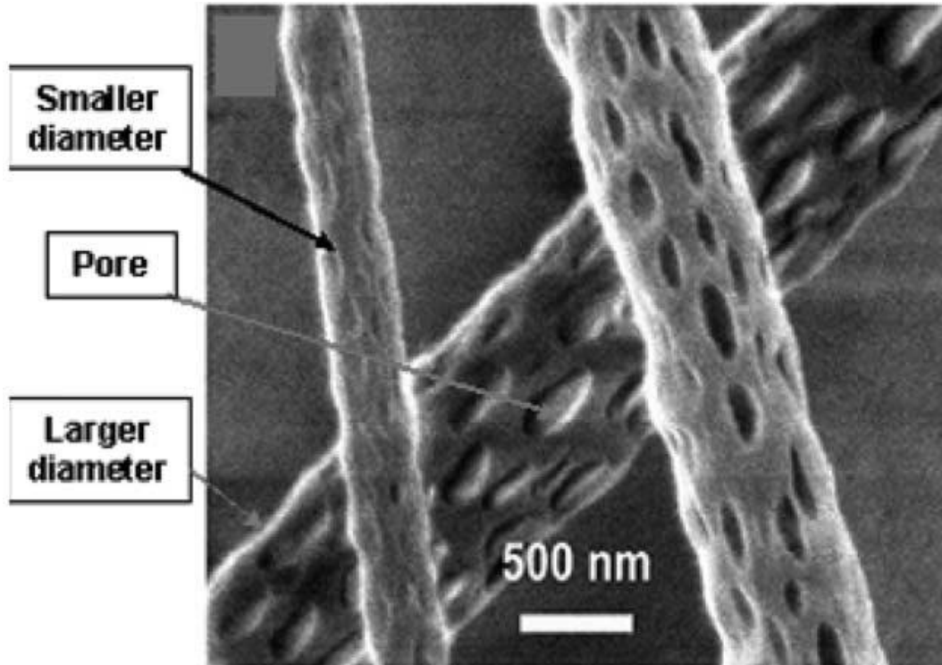
Fig. 1. PLLA nanofibers with different diameters and pores [18]
