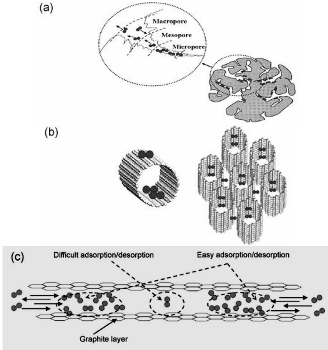
Fig.5. the mechanism of hydrogen adsorption using various carbon materials;(a): activated carbon, (b): single walled carbon nanotube, (c): graphite,
