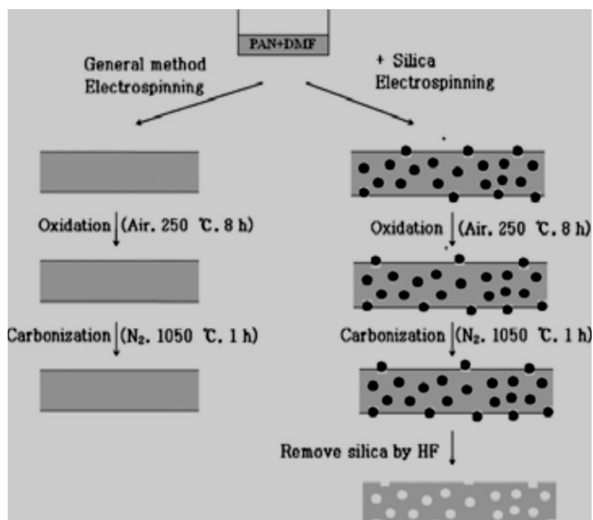
Fig. 3. The procedure of manufacturing carbon fibers and silica-activated carbon fibers.
