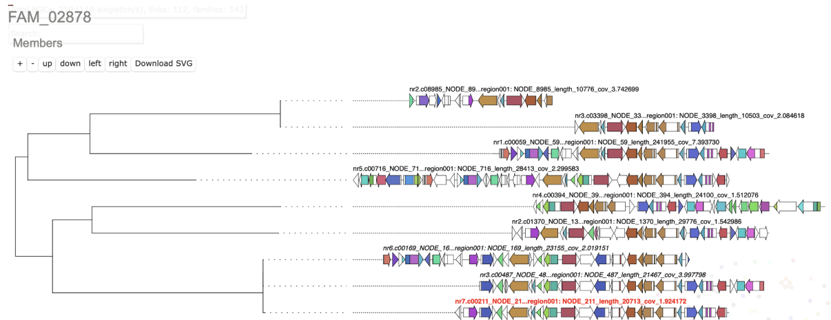
Figure S1: BiG-SCAPE clustering result depicting terpene gene cluster family containing BGC cluster from each of the soils. nr1=Podzol-O, nr2=Podzol-A, nr3=Cambisol-O, nr4=Cambisol-A, nr5=Cambisol-B, nr6=Stagnosol-O, nr7=Stagnosol-A
