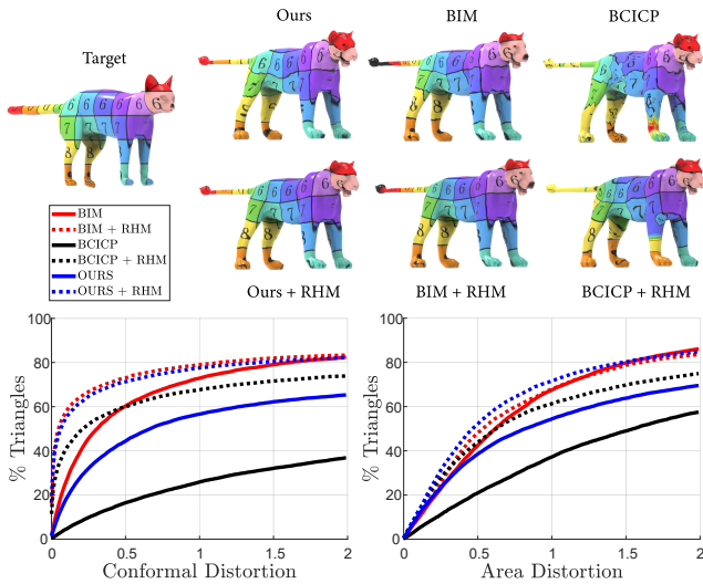
Figure 14: Sumner, qualitative and quantitative comparison with automatic methods BIM and BCICP, with and without RHM refinement. Note that we achieve conformal distortion similar to BIM, yet a better area distortion.
