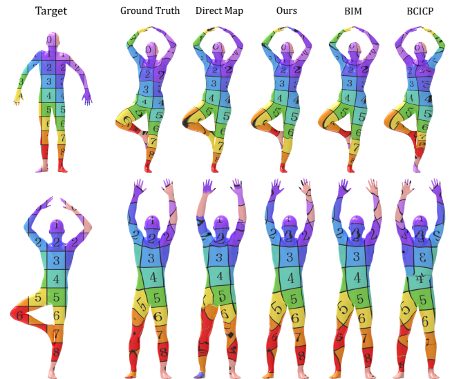
Figure 16: Map composition leads to a higher quality inter-map for non-corresponding shapes compared with computing the map directly. All maps include RHM refinement.
