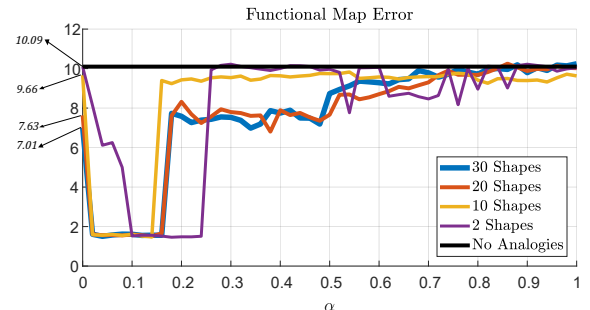
Figure 20: Functional map error for varying regularizer weight and several collection sizes. See the text for details.
