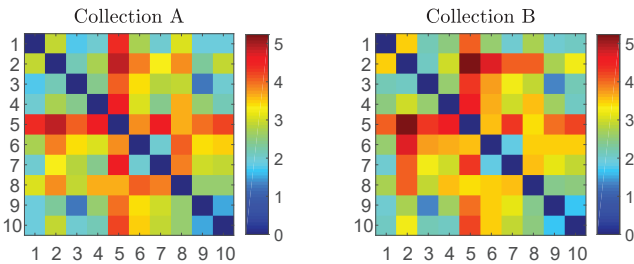
Figure 4: Distance matrices of the collections from Figure 1, for the conformal shape differences (both collections are ordered correspondingly for better visualization). Note that the cats (collection \mathcal{A} ) and the lions (collection \mathcal{B} ) have similar distance matrices, which we use for matching the collections.
