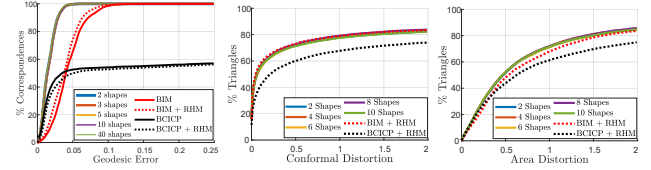
Figure 19: Varying collection size, Blend Shapes (left, without RHM) and Sumner (center and right, with RHM) datasets. We obtain a high-quality map even for collections with only 2 shapes.
