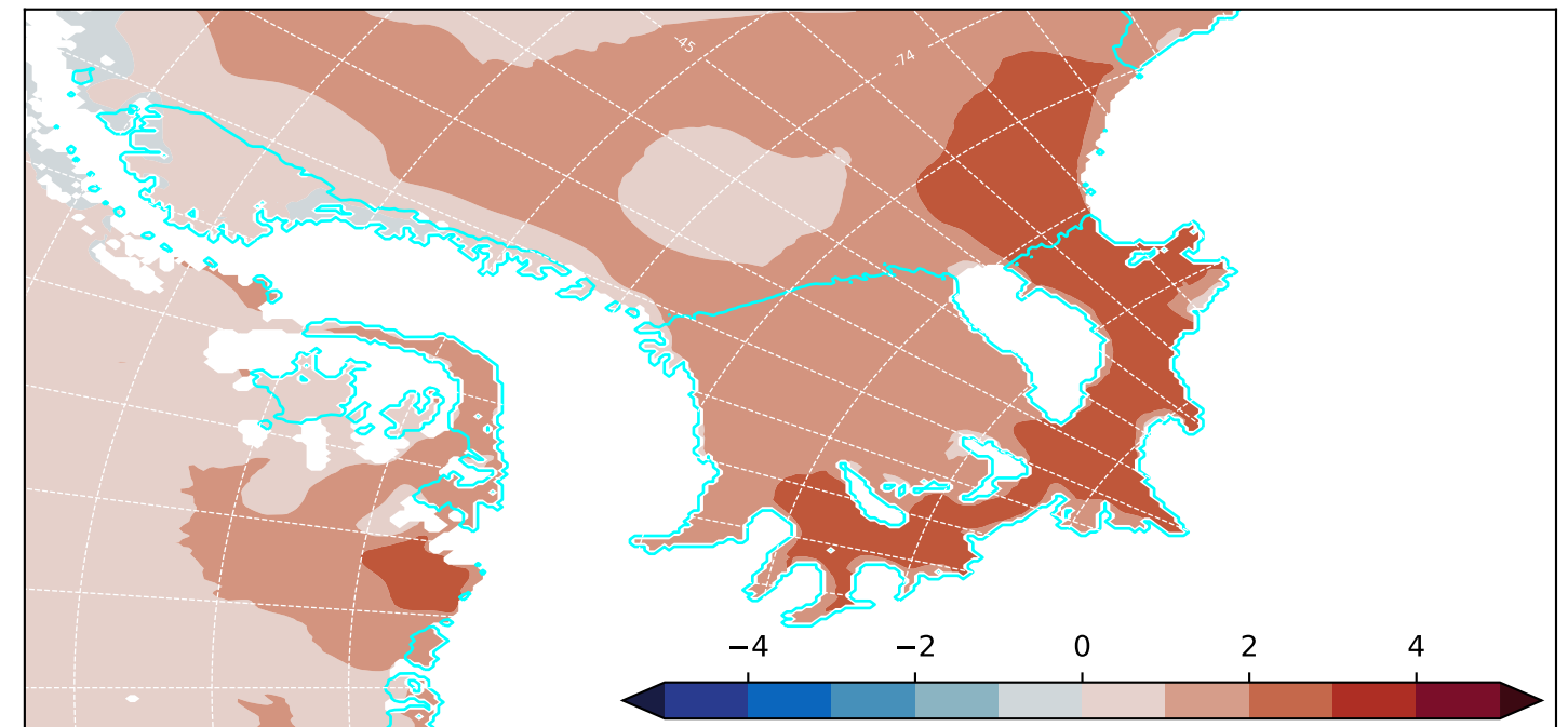
(f) Temperature anomaly, Ross Sea (NEMO eORCA025)
