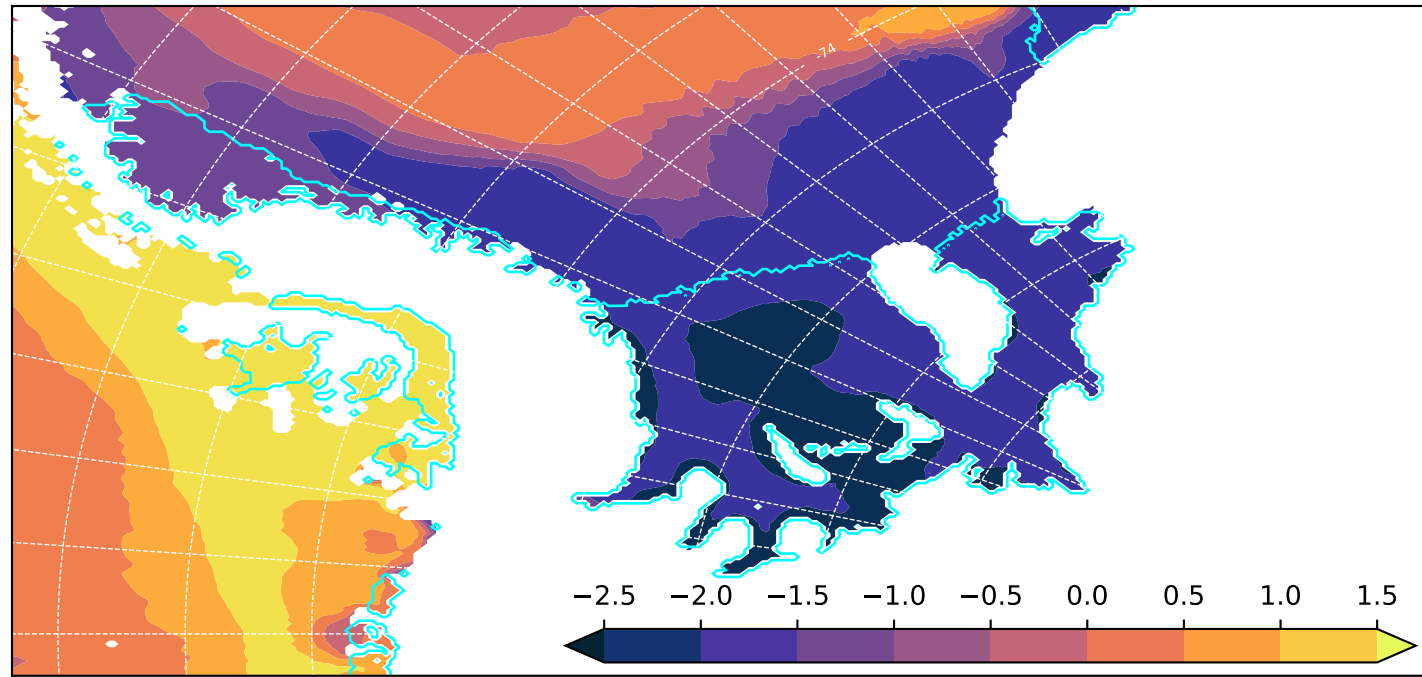
(c) Seafloor potential temperature (FESOM \sigma high)
