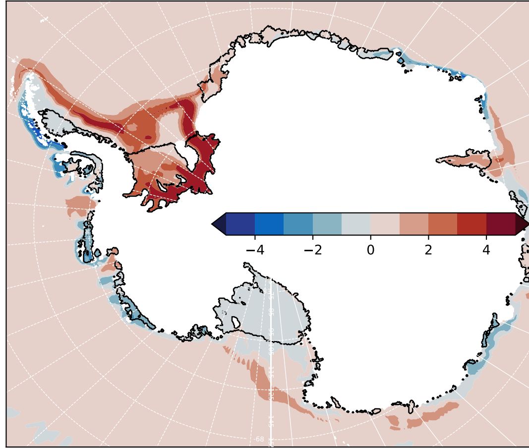
(e) Temperature anomaly (FESOM z low)
