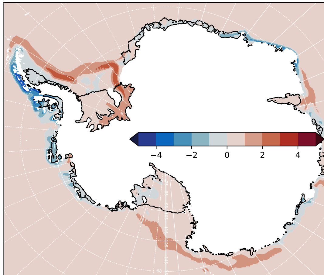
(h) Temperature anomaly (FESOM \sigma low)
