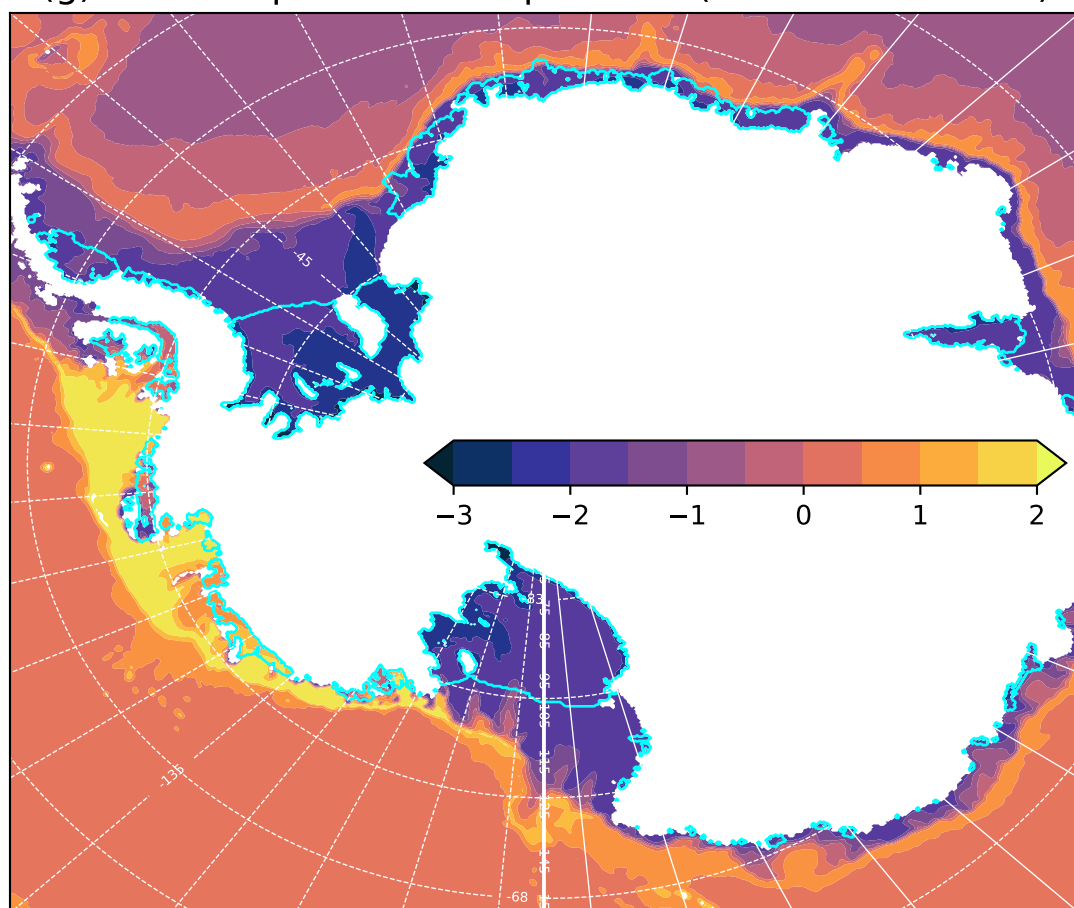
(g) Seafloor potential temperature (NEMO eORCA025)
