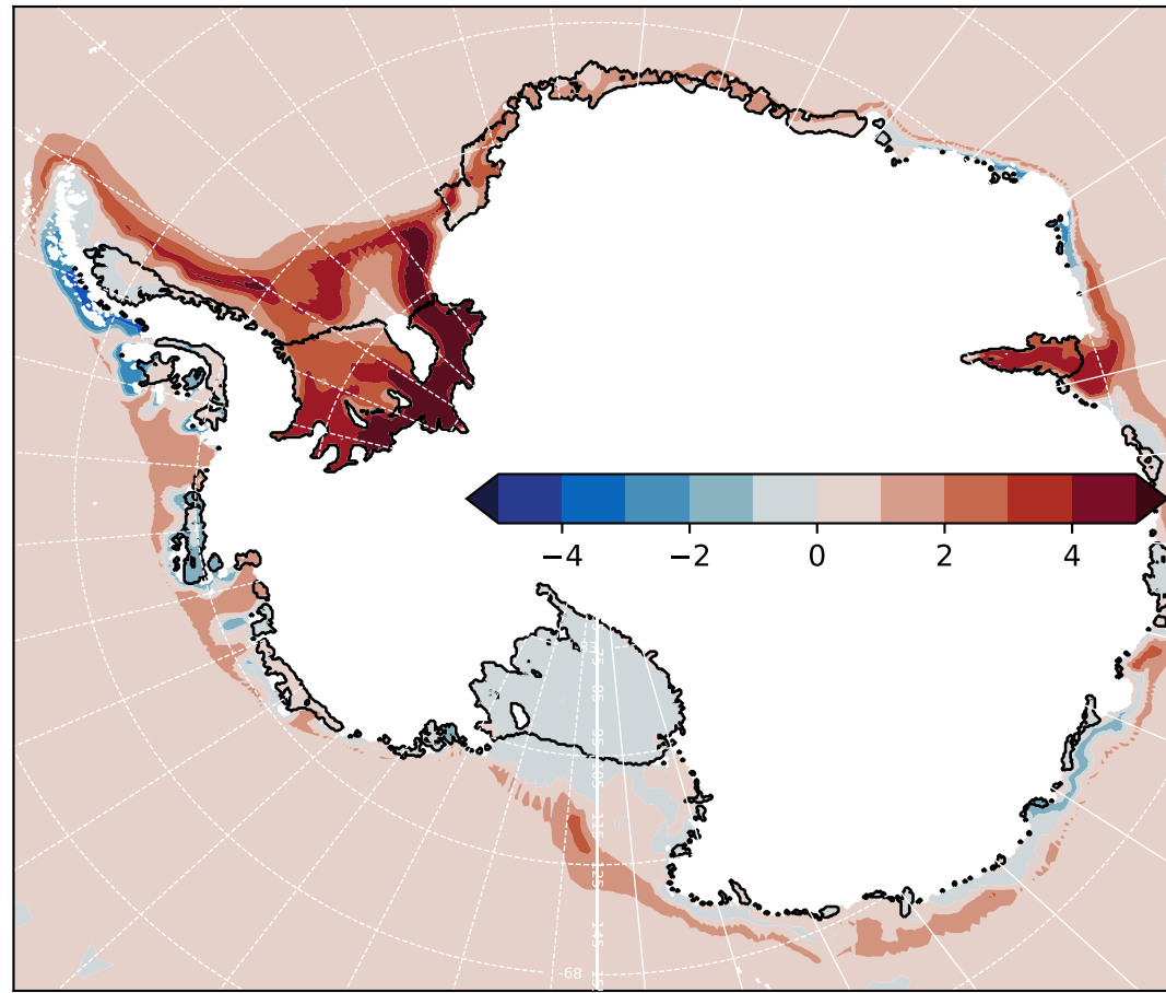
(e) Temperature anomaly (FESOM \sigma high)
