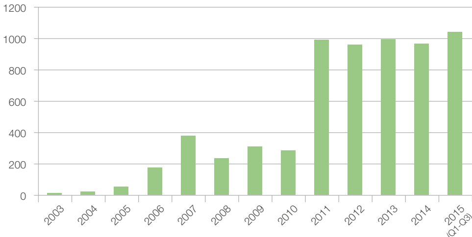
Figure 4: Incidents with counter-measures in the control area of TenneT Germany (without voltage/reactive power problems; numbers for 2015 including first to third quarter Q1-Q3)
