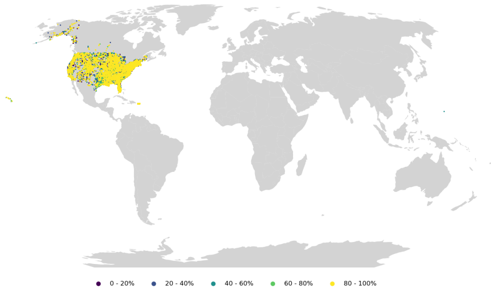
Monthly time series availability of TAN observations
