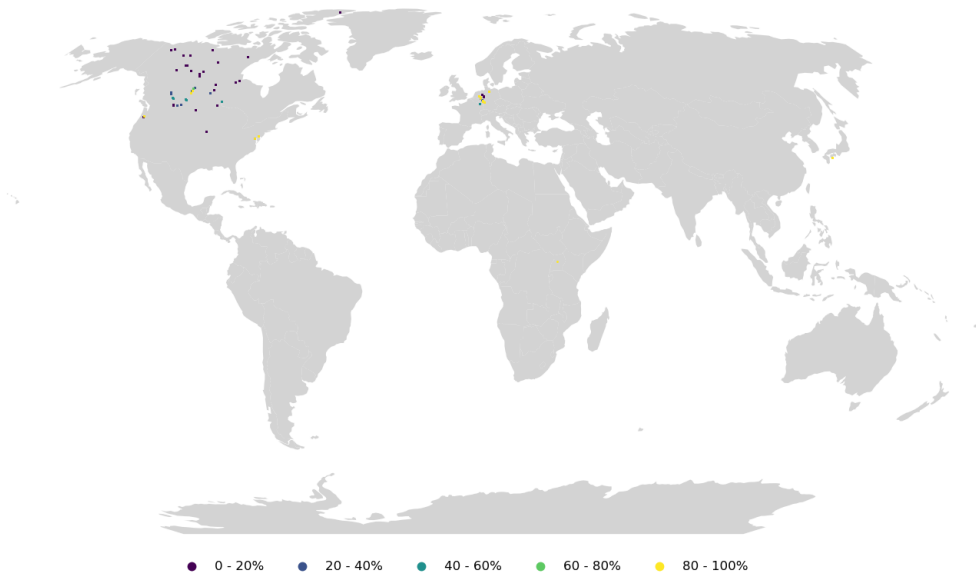
Monthly time series continuity of TPP observations
