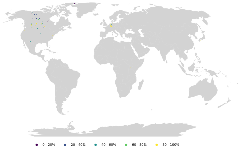
Monthly time series availability of TPP observations
