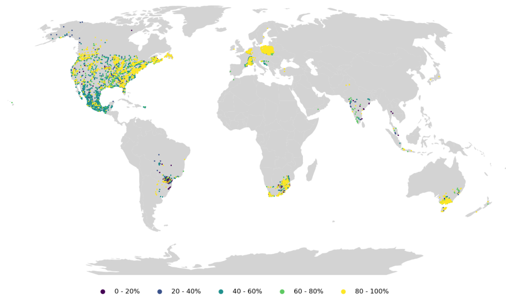
Monthly time series availability of TKN observations
