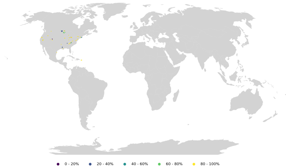
Monthly time series availability of DOP observations
